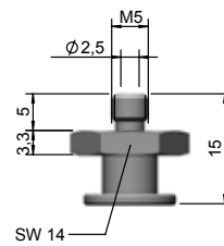
WGS-VN-G1/8 022049
