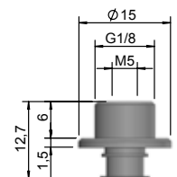
WGS-VNU-G1/8-PI2 024062
