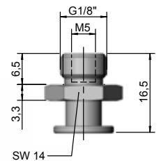
WGS-VN-G1/8 022049
